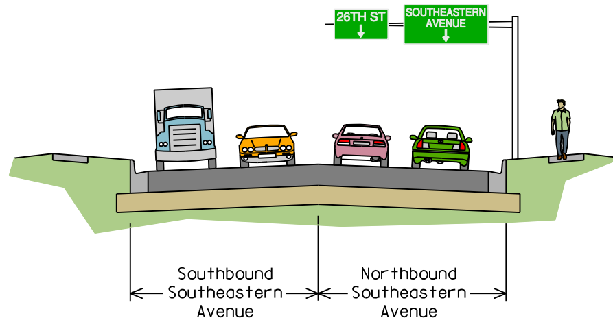
Section View Looking North
